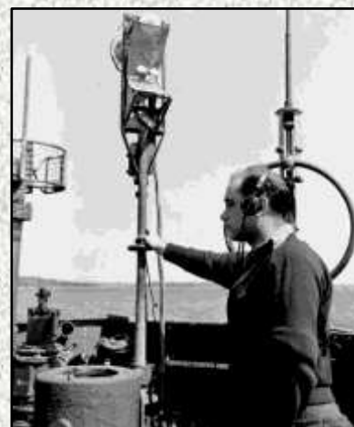
Below (B106): U 889 in May 1945, showing the newer style of direction-finding loop with a round area and aerial on top. The Tunis combination is mounted on a pole, with the horn-shaped Mücke facing away from us and the curved-shaped Fliege on the front.
