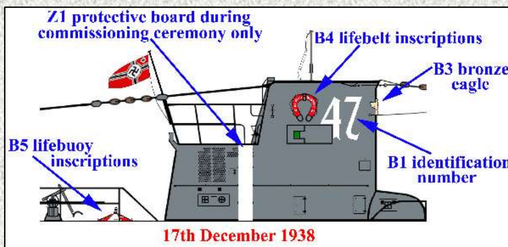
Above (A8): This drawing shows some of the features on the boat during commissioning that were removed prior to hostilities.
