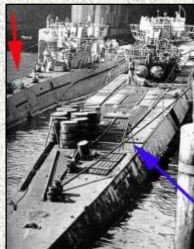
Above (B111): The blue arrow points to the rear tripods on the IXD2 U 862 while the red arrow points to the style which faced outwards on the VIIC/41 U 995.
