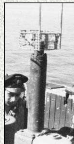
Below (B91): The Bali runddipol on U 181 at the top of periscope housing between periscopes. Some runddipols had one dipole while others had two dipoles.
