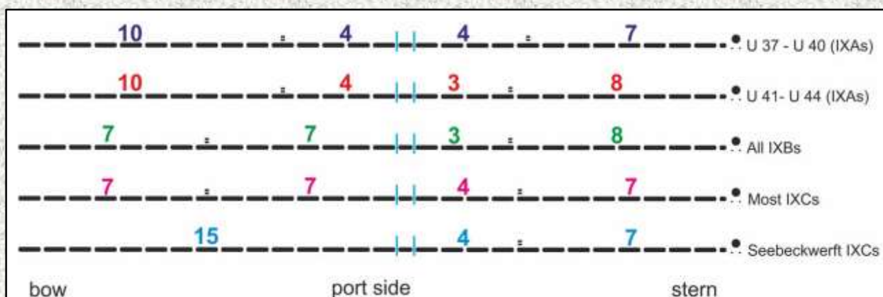
Above (B67): The position of the two sets of double footholes on IXAs, IXBs and IXCs.
