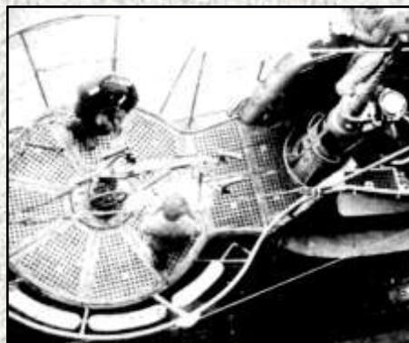
Above left (D1): Although this image is of the VIIB U 86, it provides a very good view from the rear of the typical wooden floor fitted to most Type VIIC U-boats.
