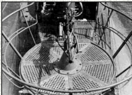
Above left (D1): Although this image is of the VIIB U 86, it provides a very good view from the rear of the typical wooden floor fitted to most Type VIIC U-boats.
