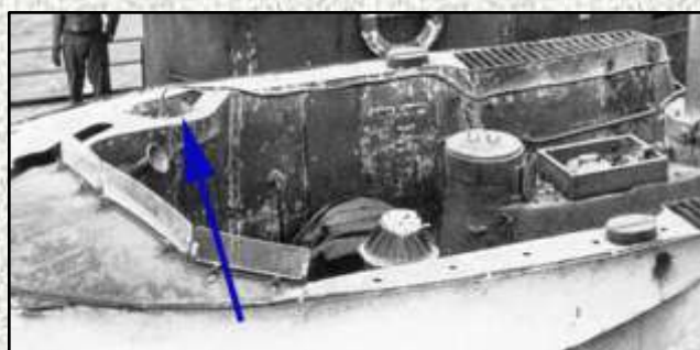
Below (B20): Another image of U 123 showing the position of the object and the cable running backwards near the top of the starboard bulwark. Note also the three areas of clear screen for the windscreen without metal frames.
