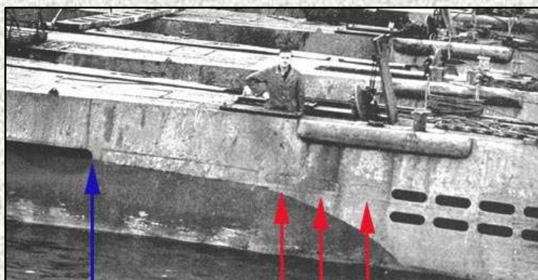
Above (C14): The three red arrows point to three vents which have a blanking plate behind them on U 776. This is addressed through a photo-etch part in AMP set 72-05. We can also see how the central drainage area begins very far back on the starboard side at the position marked with the blue arrow. A long horizontal blanking plate is present to the left of the three vents on U 776 but this was not in place on U 1023 and, it is assumed, other boats.
