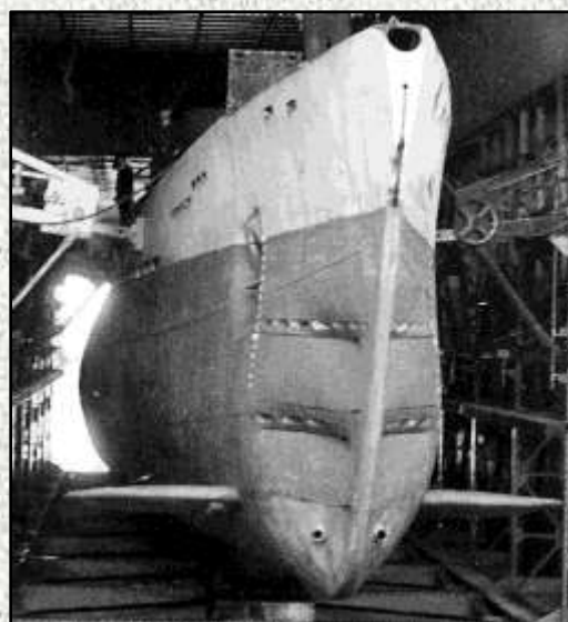
Above (B34): The two vents near the top of this unidentified boat indicate to us that it is a Type IXC. Clearly there is no S-Gerät on the stem of what could be a later war boat.
