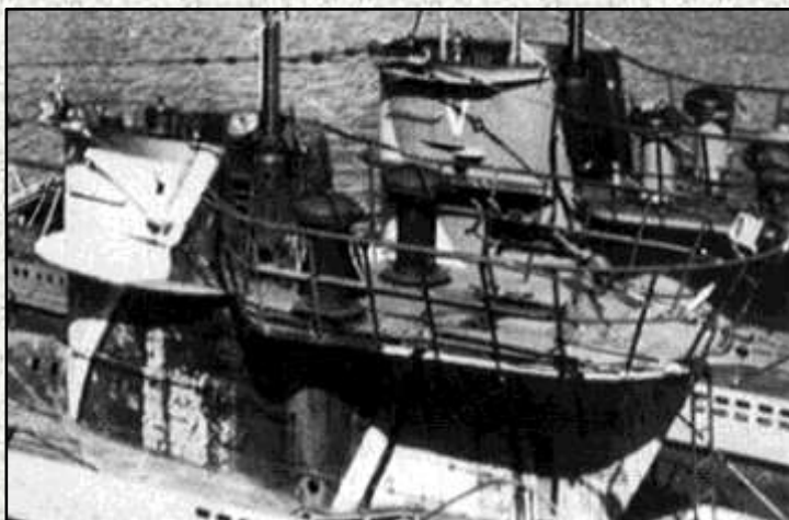
Above (D12): The Breda pods can be seen in the extended position on U 73 (left) and U 561 (right). These could be retracted into the tower floor, with only the lids being exposed.
