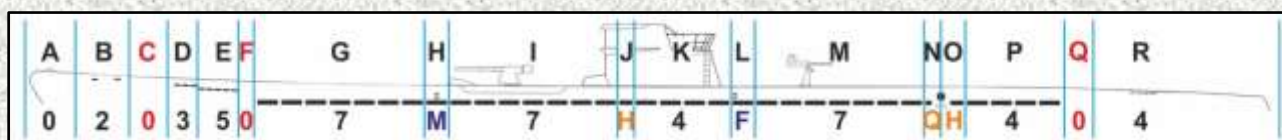
Above right (B68): F, M and R (front, middle, rear) denote the position of the footholes above the main vents. Q, H and T are used to denote for quarter-length, half-length and three-quarter-length main vents.
