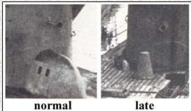
Above (C41a & C41b): The old magnetic compass fairing was very different to the late Askania fairing.
