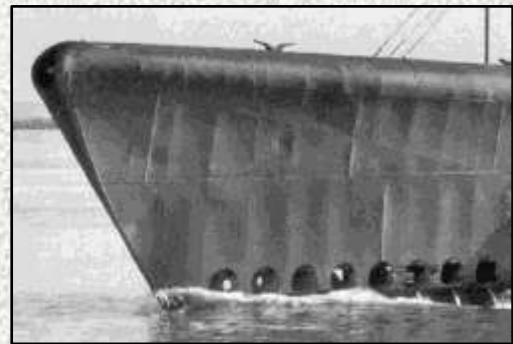
Above (H18): Oil canning on a Gato.
