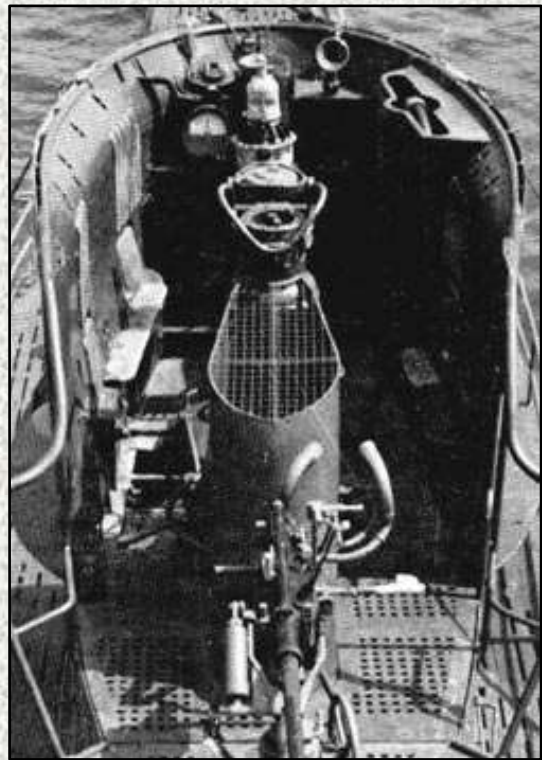
Above (C7): The teardrop shaped fairing behind the attack periscope base on the VIIB U 86. The grill is at the top of the fairing.
