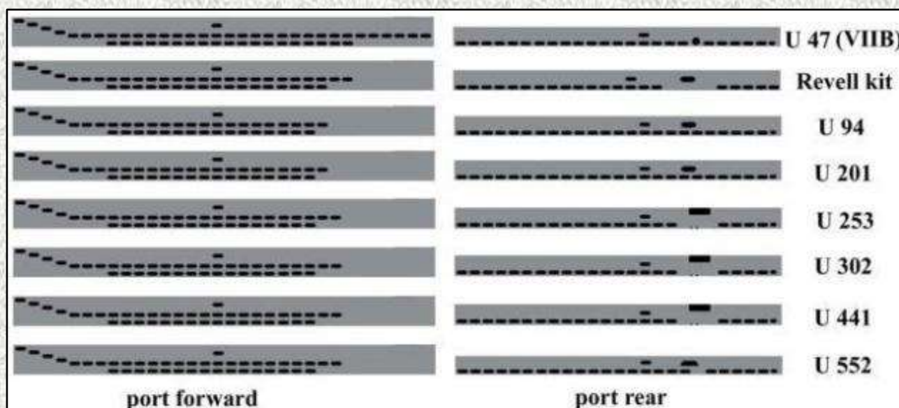
Above: The port side of the main groups of free-flooding vents for six VIICs, one VIIB and the Revell kit.
