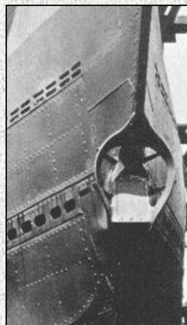
Above (C25): The S-Gerät bow device (S-G) on the stem of U 559.
